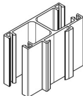
Type SDV2 – standard, double (groove centre)
