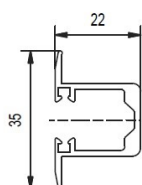
Type Z – hidden
