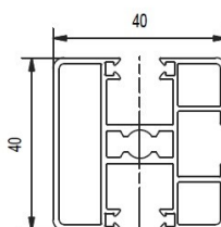
Type HDV – square, double
