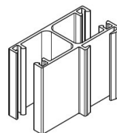
Type SDV – standard double (groove side)
