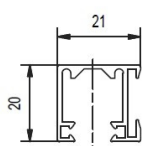
Type S – standard, single
