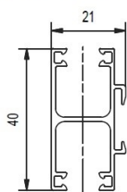
Type SDV2 – standard, double (groove centre)
