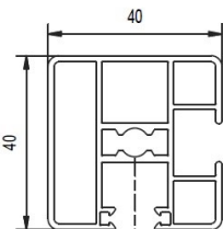
Type H – square, single
