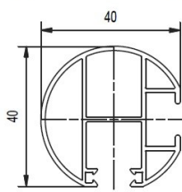
Type K – round, single
