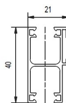
Type SDV – standard double (groove side)
