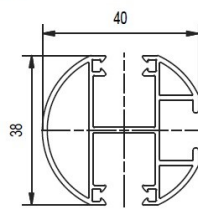
Type KDV – round, double
