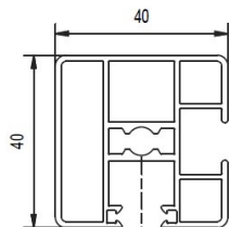
Type H – square, single
