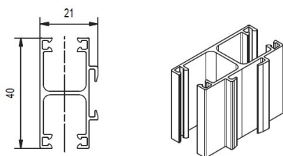
Type SDV2 – standard, double (groove centre)
