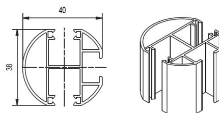
Type KDV – round, double
