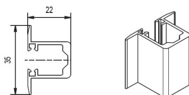
Type Z – hidden
