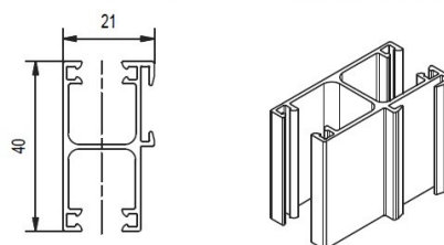
Type SDV – standard double (groove side)
