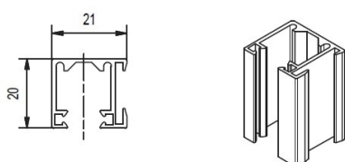
Type SDV2 – standard, double (groove centre)
