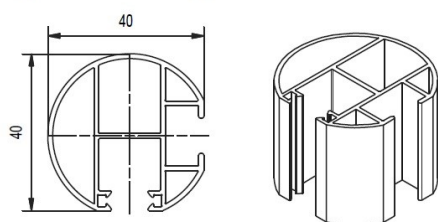
Type K – round, single
