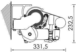
Montaggio a parete con staffa estrusa Wall installation with extruded bracket
